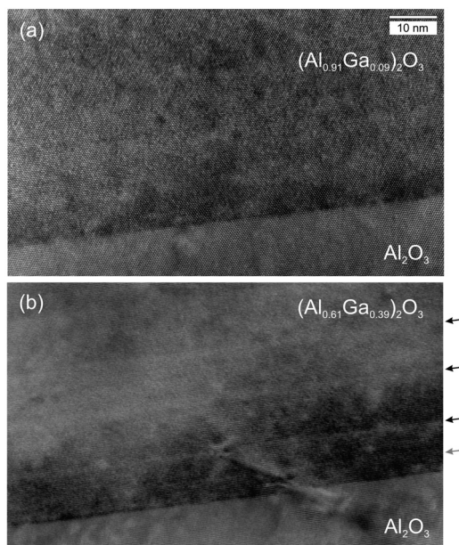
Fig. 1 Cross-sectional TEM images of the substrate/film interface region of two \alpha -( \text{Al}_x\text{Ga}_{1-x} ) _2\text{O}_3 thin films on (01.2) \text{Al}_2\text{O}_3 with (a) x = 0.91 ( [0\bar{1}.1] viewing direction) and (b) x = 0.61 ( [\bar{1}2.0] viewing direction). The arrows in panel (b) indicate anomalies in the cation ratio.
