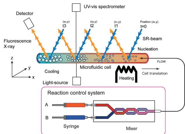
Fig. 20 "Schematic principle of the in situ XAFS experimental set-up using a microfluidic cell. Fluorescence yield spectra record at positions ( x , y ) along a microreactor channel provide time-dependent XAFS spectra. In the present reaction, precursor flows (TOP-Se and Cd stock solution) are mixed before introducing to a heated microchannel." 43 Reproduced with permission from ref. 43. Copyright 2011 International Union of Crystallography.
