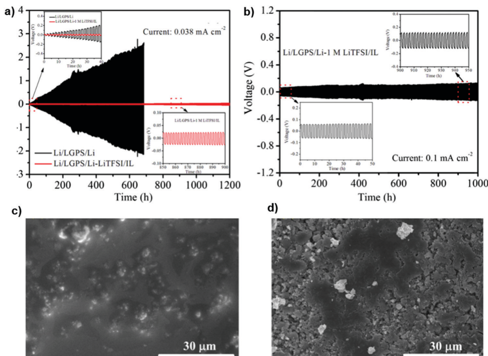
Fig. 21 (a) Galvanostatic cycling curves of cells with and without 1 M \text{LiTFSI/IL} at 0.038 \text{ mA cm}^{-2} and (b) the cell with 1 M \text{LiTFSI/IL} . SEM images after long-term Li stripping/plating cycles for the cells (c) with and (d) without 1 M \text{LiTFSI/IL} . Image reprinted with permission from ref. 135. Copyright © 2019, American Chemical Society.
