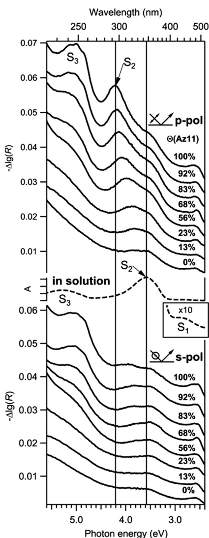
Fig. 3 Series of p- and s-polarized differential reflectance (DR) spectra of SAMs for different Az11 coverages \theta (angle of incidence 45°, offsets were added). Schematic drawings indicate the orientation of the electric field vector of the incident light. An absorbance spectrum of trans -Az11 in methanol (middle, dashed) is plotted for comparison. The inset shows the upsampled S 1 absorption band in solution. Reprinted (adapted) with permission from T. Moldt, D. Brete, D. Przyrembel, S. Das, J. R. Goldman, P. K. Kundu, C. Gahl, R. Klajn and M. Weinelt, Langmuir , 2015, 31 , 1048–1057. Copyright (2015) American Chemical Society. 92
