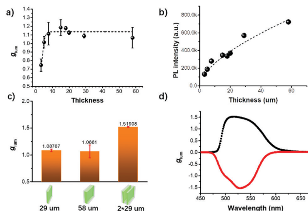
Fig. 3 Plots of (a) maximum g_{lum} , \lambda_{ex} = 380 nm, and (b) photoluminescence intensity at 524 nm, \lambda_{ex} = 447 nm laser, versus the various thicknesses of the N*LC. (c) g_{lum} values of N*LC loaded by a 29 \mu\text{m} single layer, a 58 \mu\text{m} single layer and double 29 \mu\text{m} layers cell, respectively. (d) The positive and negative g_{lum} curves are responsible for R811 and S811 doped N*LC in the double 29 \mu\text{m} layer cell, respectively. C6:R/S-811:SLC1717 = 1:47:100 weight ratio, \lambda_{ex} = 380 nm.
