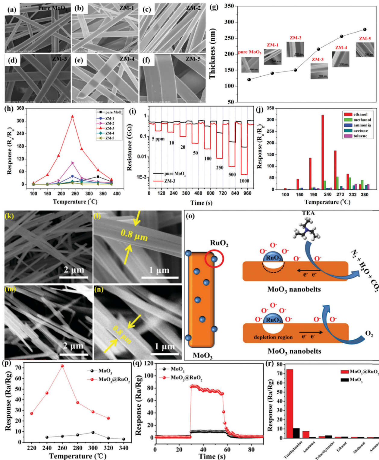
Fig. 1 (a–f) FESEM images of pure \text{MoO}_3 NBs and ZM-1–ZM-5; (g) the average thicknesses of pure \text{MoO}_3 NBs and Zn-doped \text{MoO}_3 NBs; (h) gas sensing responses of the sensors based on pure \text{MoO}_3 NBs and Zn-doped \text{MoO}_3 NBs to 1000 ppm ethanol at different OTs; (i) response and recovery curves of the sensors based on pure \text{MoO}_3 NBs and ZM-3 to different concentrations of ethanol at the OT of 240 °C; (j) cross-sensitivity to various gases at different temperatures; reproduced with permission from ref. 103, copyright 2017 Elsevier. (k and l) FESEM images of pure \text{MoO}_3 NBs; (m and n) FESEM images of \text{RuO}_2/\text{MoO}_3 NBs; (o) schematic diagram of the possible gas sensing mechanisms of \text{RuO}_2/\text{MoO}_3 NBs; (p) response to 10 ppm TEA gas versus OT; (q) response transient to 10 ppm TEA at 300 °C; (r) responses of pristine and \text{RuO}_2/\text{MoO}_3 NBs gas sensors to different gases (10 ppm) at 300 °C. Reproduced with permission from ref. 60, copyright 2019 Elsevier.
