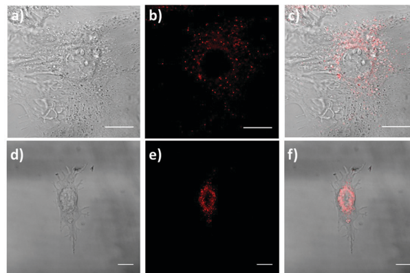
Fig. 9 Fluorescence images of subcellular localization of 1 (a–c, \lambda_{\text{exc},2P} = 720 nm, \lambda_{\text{em}} = 450\text{--}700 nm) and 2 (d–f, \lambda_{\text{exc},2P} = 740 nm, \lambda_{\text{em}} = 450\text{--}700 nm) in MEF cells. (a and d) Brightfield in MEF cells. Fluorescence images of compound 1 (b) and compound 2 (e). Brightfield and fluorescence merged images of compound 1 (c) and compound 2 (f). Scale bar: 15 \mu\text{m} .
