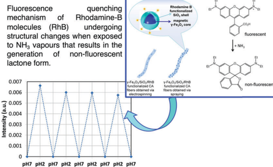
Reversibility of the pH-dependent on-off-on fluorescence intensity profile of electrospun magnetic fibers. The RT of the pH sensor was 30 s.
