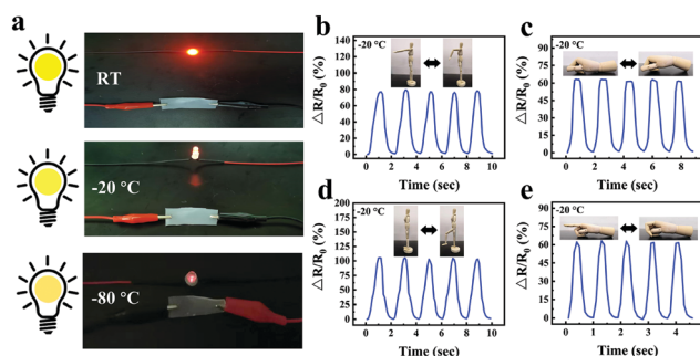
Fig. 11 (a) The LED lighting conditions of the gelatin/pHEAA/Gly/LiCl organohydrogels at room temperature, -20\text{ }^{\circ}\text{C} and -80\text{ }^{\circ}\text{C} . (b) The changes in the relative resistance of the gelatin/pHEAA/Gly/LiCl DN organohydrogel strain sensor were used to monitor the movement of an (b) elbow, (c) wrist, (d) knee and (e) finger at -20\text{ }^{\circ}\text{C} .
