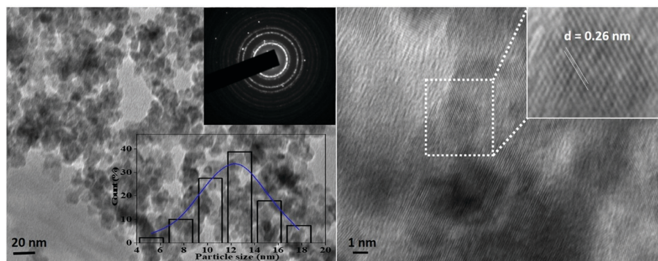
Fig. 6 TEM and HR-TEM images with inset images showing the corresponding SAED image and the size distribution histogram fitted by Lorentzian function of V 2 O 5 nanoparticles prepared via the hydrothermal method.
