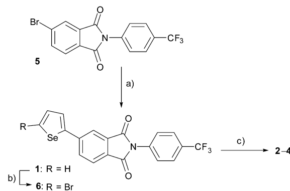
Scheme 1 Preparation of target PIs 1–4 and bromine substituted precursor 6. Reagents: (a) \text{Pd}(\text{PPh}_3)_4 , 2-(tributylstannyl)selenophene (y, 80%), (b) NBS (93%), (c) \text{Pd}(\text{PPh}_3)_4 , 2-(tributylstannyl)selenophene for 2 (60%); 5-tributylstannyl-2,2'-biselenophene for 3 (45%); tributylstannylbenzene for 4 (63%).
