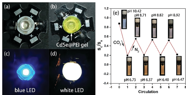
Fig. 5 Blue LED beam before (a) and after (b) coating CdSe@PEI gel. (c and d) The emission color of the LED beams after powering on. (e) The changes of emission color and pH of a CdSe@PEI aqueous solution by cyclical bubbling CO 2 or N 2 into the solution (irradiated by a UV lamp of \lambda_{\text{ex}} = 365 \text{ nm} ).
