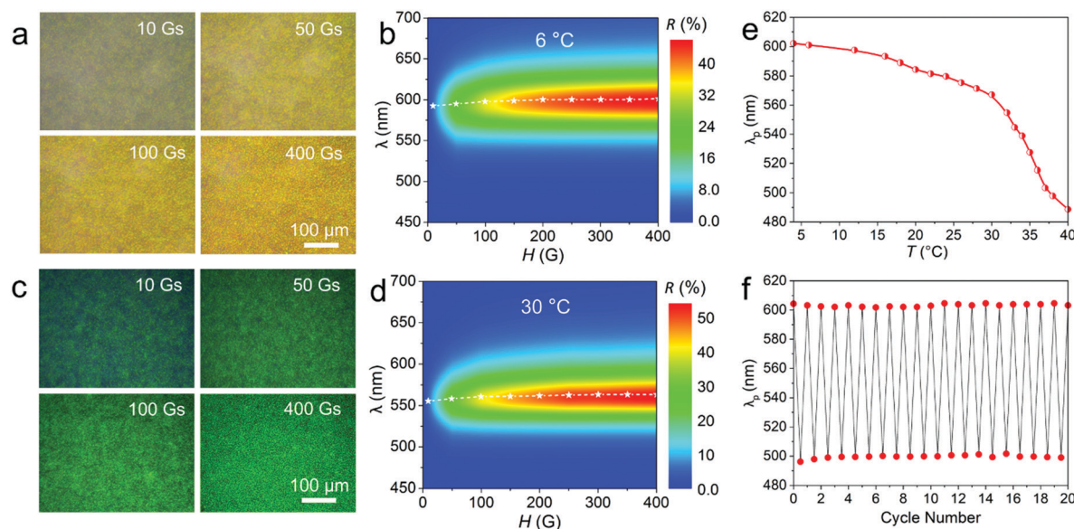
Fig. 2 The dual responsive optical properties of the typical \text{Fe}_3\text{O}_4\text{@PVP@PNIPAM} flexible PNCs. (a and c) Dark-field optical microscopy images, and (b and d) 2D contour maps of the reflection spectra obtained under different H and T values. (a and b) 6 °C; (c and d) 30 °C. (e) Diffraction wavelength as a function of T . (f) Cycling performance showing the variation in diffraction peaks between 4 and 38 °C over 20 cycles. The magnetic field direction in (a and c) is parallel to the observation direction.
