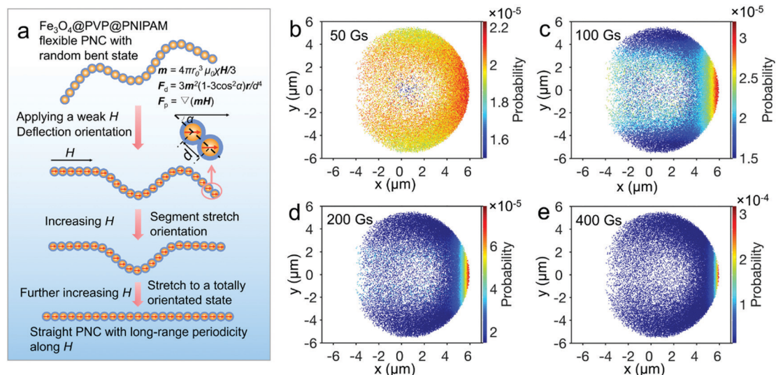
Fig. 4 (a) Schematic illustration for the orientation process of a flexible PNC under H . (b–e) The calculated probabilities of different conformations shown by 50 000 flexible PNCs under different H values.
