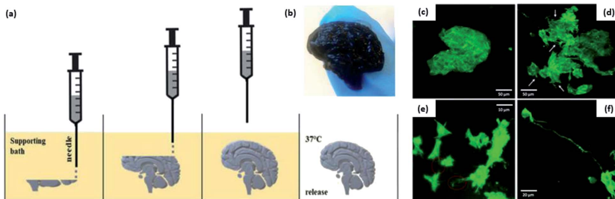
Fig. 16 (a) Schematic of the FRESH 3D-bioprinting technique; (b) FRESH 3D-bioprinted brain scaffold with an intricate structure; confocal imaging of (c) neural cells cultured on the brain scaffold printed with 100% CNF without any observed differentiation; (d) cells cultured on a conductive brain scaffold without any observed differentiation but more neurites; (e) visible interaction within the cells cultured on a conductive ink; (f) differentiation between the cells cultured on a conductive ink observed with a long neurite [adapted with permission from Bordoni et al. 2020, 240 Copyright © MDPI].
