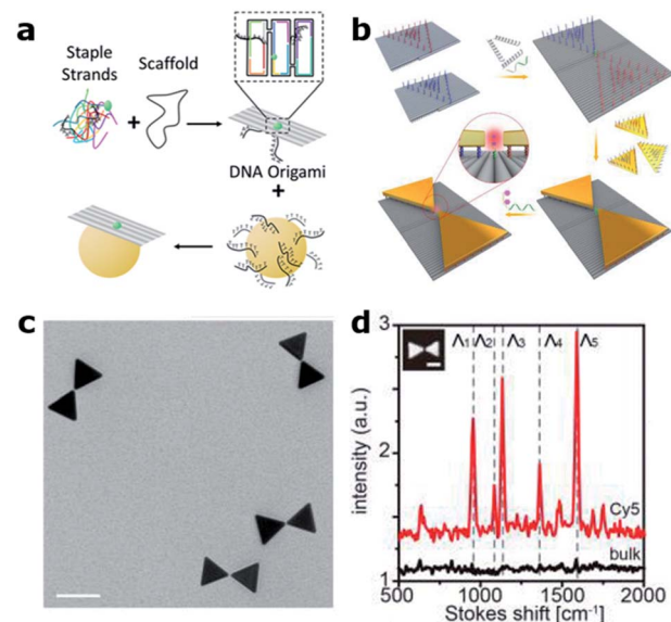
Fig. 4 DNA origami based nanocavities. (a) Basic principle: a “long” ss-DNA sequence (Scaffold) is folded with the help of hundreds of “short” ss-DNA sequences into the predesigned shape. MNPs, previously functionalized with DNA, can be incorporated through DNA hybridization. (b) Bowtie antennas self-assembled onto DNA origami structures fabricated based on two rectangular DNA origami structures. A single Cy5 Raman active molecule is incorporated at the bowtie hotspot. (c) Corresponding TEM image (scale bar 50 nm) and (d) Raman spectra of an individual bowtie with a single Cy5 (red) and a bulk solution of Cy5 (black). (b)–(d) have been reproduced from ref. 76 with permission from Wiley, copyright 2018.
