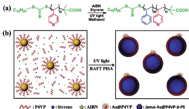
Scheme 1 (a) Synthesis of P4VP- b -PS block copolymers. (b) The fabrication of Janus Au@BCP nanoparticles by UV light-initiated RAFT PISA. UV light intensity: I_{365 \text{ nm}} = 2.50 \text{ mW cm}^{-2} ; irradiation time: 9 h, 25 °C.
