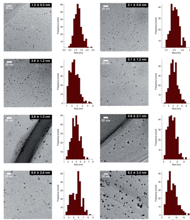
Fig. 1 TEM images of AuPd:PVP nanoalloys.
