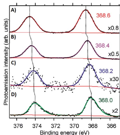
Fig. 9 Ag 3d peak doublet for (A) Ag + -DNA complexes, (B) AgNO 3 salt, (C) HPLC-purified fluorescent Ag N -DNAs (which combine both neutral and cationic Ag) and (D) metallic Ag nanoparticles. Adapted from Volkov, et al. , (ref. 158) with permission from the American Chemical Society. Copyright 2017.
