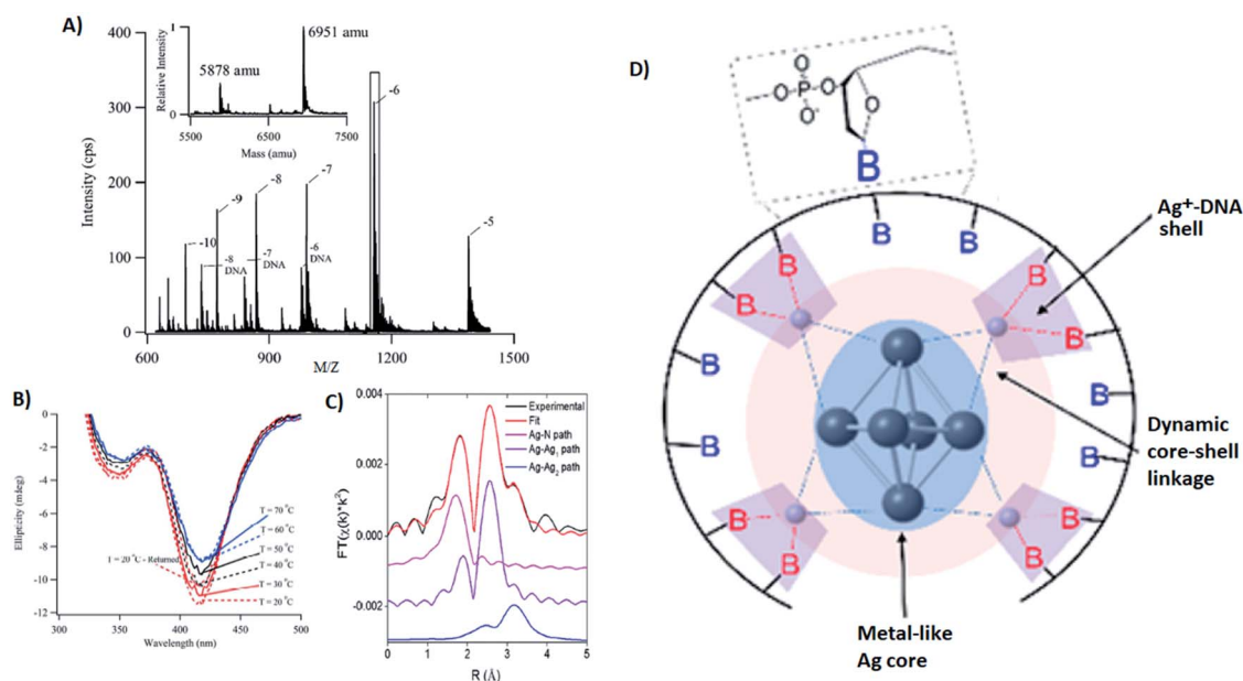
Fig. 8 (A) Mass spectrum of 20-base DNA-templated \text{Ag}_N . The peaks labeled -10 to -5 correspond to the ions of the \text{Ag}_N\text{-DNA} , while the peaks labeled -8 DNA to -6 DNA are ascribed to the ions of the bare DNA strand. The inset shows the zero-charge spectrum that identifies the native DNA at 5878 amu and the DNA with 10 Ag at 6951 amu. (B) CD spectra of \text{Ag}_N\text{-DNAs} at different temperatures. (C) Ag K-edge EXAFS trace of the solution state \text{Ag}_N\text{-DNAs} . The experimental data (black) was fitted (red) with three individual scattering paths (magenta, purple and blue) displayed separately. (D) Suggested \text{Ag}_N\text{-DNA} structure after combining all information from MS and EXAFS measurements. 130 Adapted from Petty, et al. , (ref. 130) with permission from the American Chemical Society. Copyright 2016.
