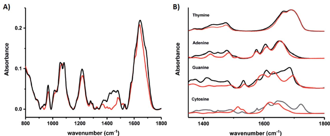
Fig. 10 IR spectra of (A) bare DNA (black) and red-emitting Ag N -DNA (red) and (B) ss-DNA homopolymers of all four DNA nucleobases with (red) or without (black) Ag(I). Adapted from Schultz, et al. , (ref. 159) with permission from The Royal Society of Chemistry.
