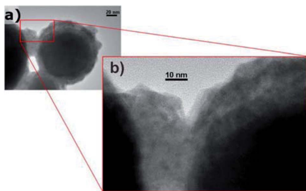
Fig. 9 TEM images of self-encapsulated Sn@SnO 2 particles. Reproduced from ref. 90. Published by Springer Nature. Copyright 2017.
