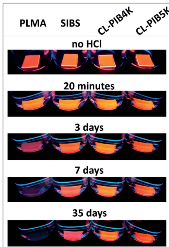
Fig. 5 Photographs of the composites of CZIS QDs-in-polymers taken under UV-light before and after the addition of 5 M solution of HCl. Some distortions in the photos are related to the lens effect of the glass vials filled with HCl solution.
