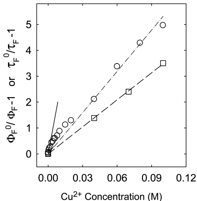
Fig. 6 For CS330, the quenching of fluorescence intensities (circle, solid line from fitting the data up to Cu^{2+} concentration of 10^{-3} M, and dash-dot line from a global fit of all data) and lifetimes (square, dash line for the best fit).
