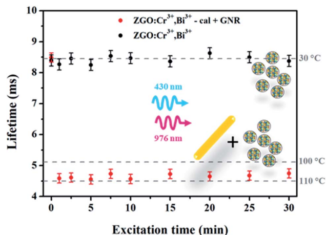
Fig. 3 Variation of the luminescence lifetime of ZGO-NTh (black) and ZGO-NTh + GNR (red) according to the laser diode excitation time.
