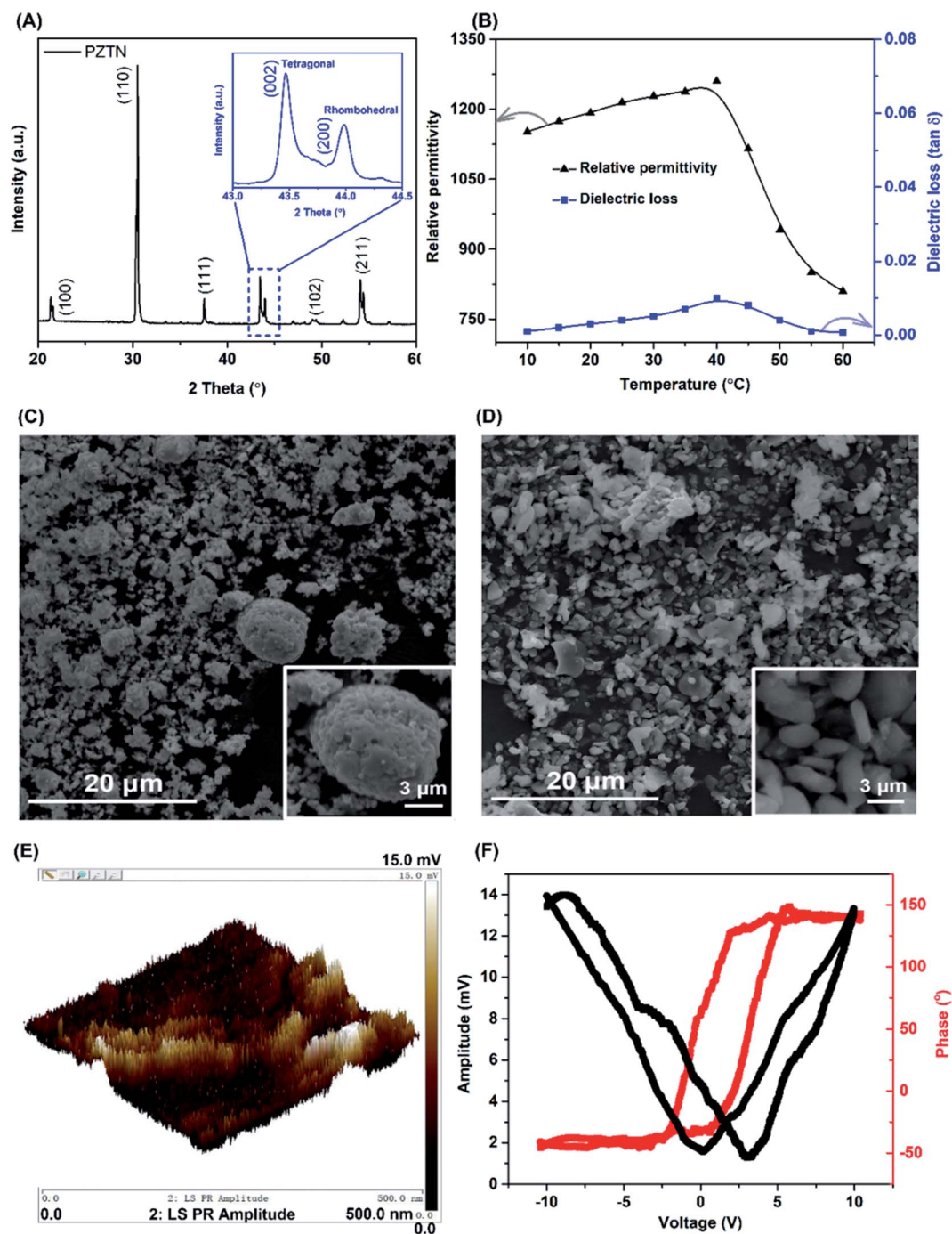
Fig. 3 (A) XRD pattern of Nb-doped PZT powders (PZTN) powders. (B) Relative permittivity as a function of the temperature. SEM images of (C) PZTN and (D) \text{Al}_2\text{O}_3 (control) powders. PFM spectrum on the local evidence of the existence of ferroelectricity in the Nb-doped PZT powders (E) out-of-plane PFM amplitude and (F) local hysteresis loop behaviour for the amplitude and phase.
