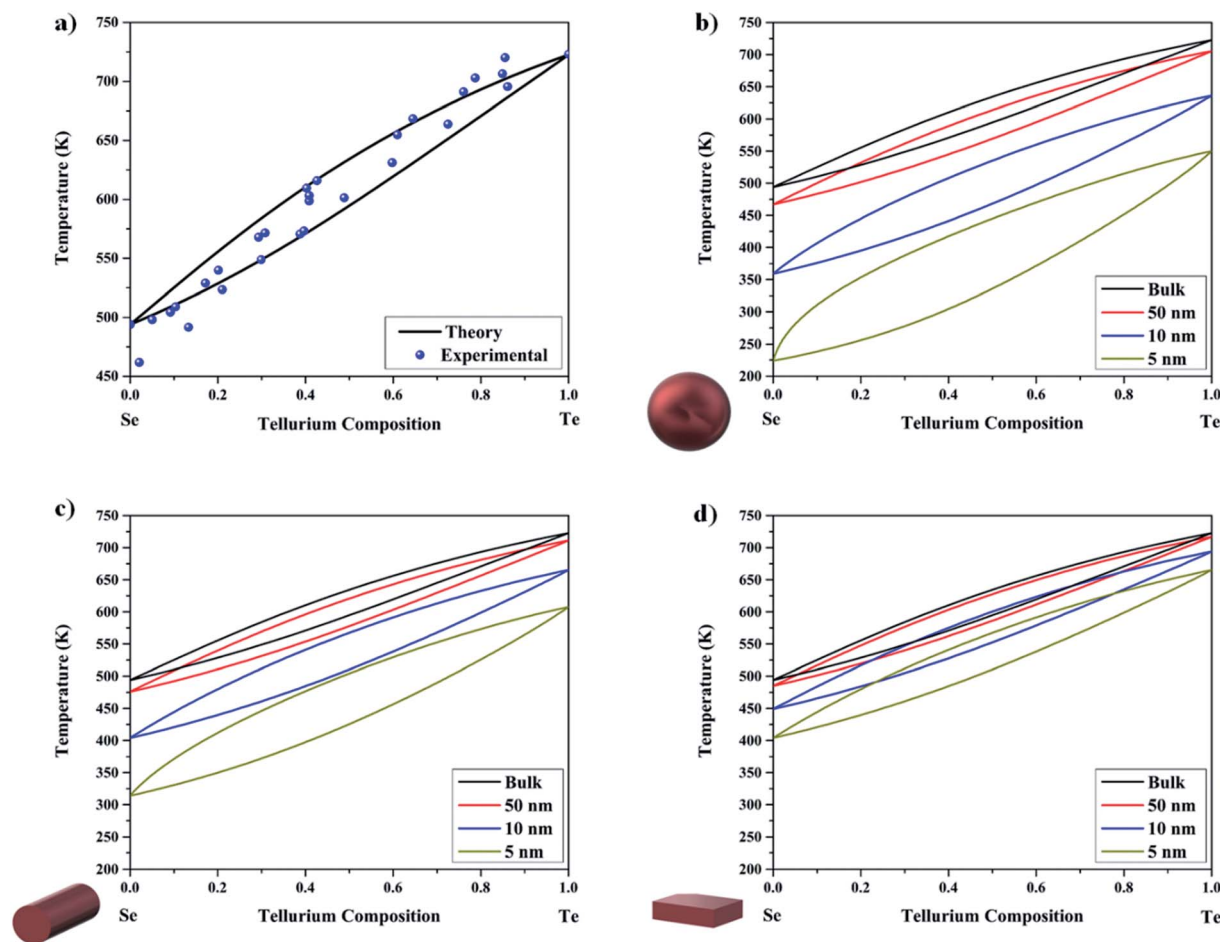
Fig. 2 (a) Binary phase diagram of the bulk \text{Se}_{1-x}\text{Te}_x alloy displaying the solidus – liquidus curves (eqn (1)). Experimental data points are taken from ref. 81. Binary phase diagram for the \text{Se}_{1-x}\text{Te}_x alloy displaying the solidus – liquidus curves (eqn (1) and (2)) at the nanoscale (50, 10 and 5 nm) for the (b) sphere, (c) wire, and (d) film morphologies.
