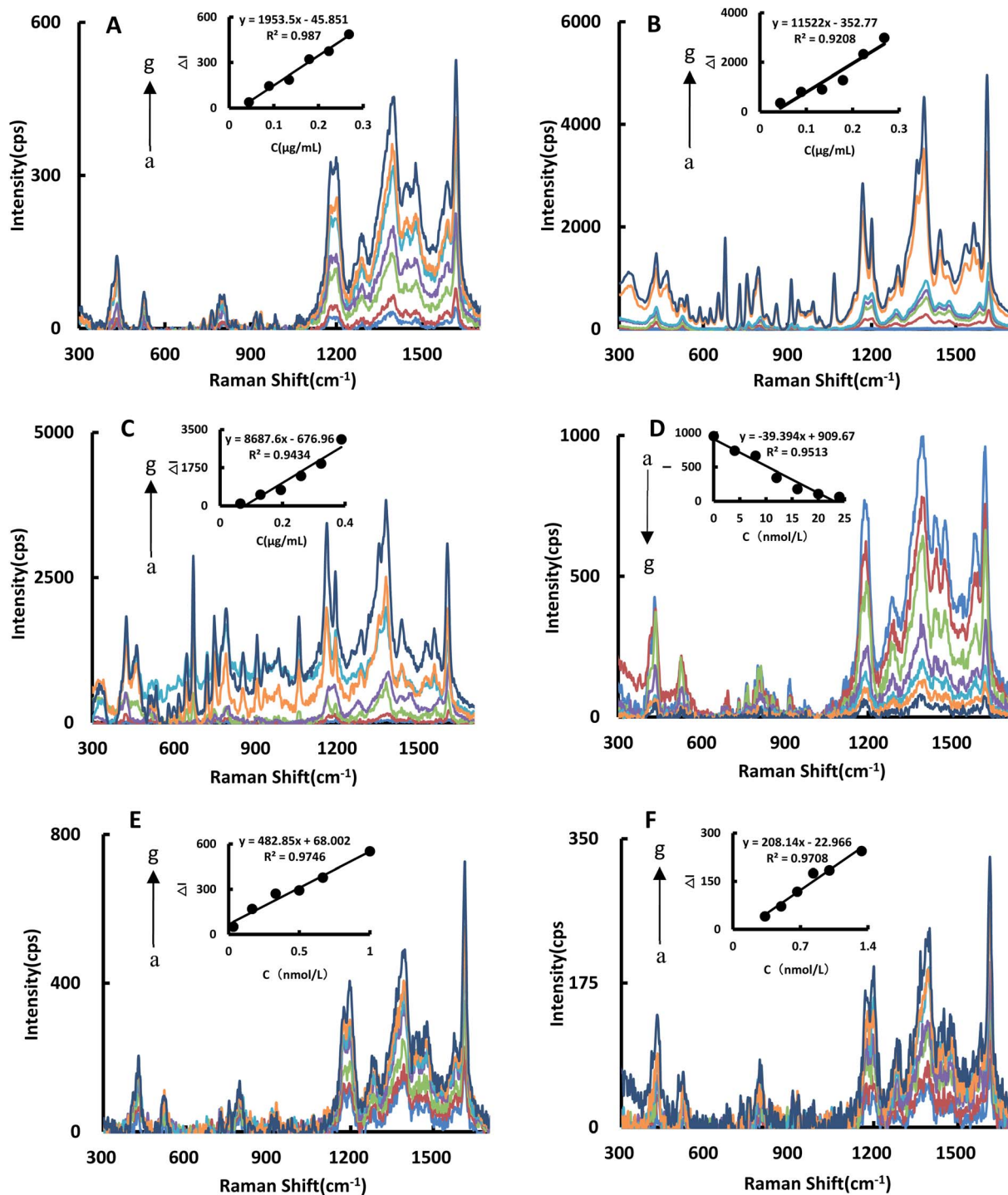
Fig. 5 SERS spectra (A): 0.067 \text{ mg mL}^{-1} \text{ HAuCl}_4 + 0.67 \text{ mmol L}^{-1} \text{ HCl} + 3 \text{ mmol L}^{-1} \text{ CHO}_2\text{Na} , (a–g) represent 0, 0.044, 0.089, 0.134, 0.179, 0.223 and 0.268 \text{ } \mu\text{g mL}^{-1} BTPD, respectively. (B): 0.067 \text{ mg mL}^{-1} \text{ HAuCl}_4 + 0.67 \text{ mmol L}^{-1} \text{ HCl} + 3 \text{ mmol L}^{-1} \text{ CHO}_2\text{Na} , (a–g) represent 0, 0.044, 0.089, 0.134, 0.179, 0.223 and 0.268 \text{ } \mu\text{g mL}^{-1} AuBTPD, respectively. (C): 0.067 \text{ mg mL}^{-1} \text{ HAuCl}_4 + 0.67 \text{ mmol L}^{-1} \text{ HCl} + 3 \text{ mmol L}^{-1} \text{ CHO}_2\text{Na} , (a–g) represent 0, 0.065, 0.129, 0.194, 0.259, 0.323 and 0.388 \text{ } \mu\text{g mL}^{-1} AuNPs, respectively. (D): 0.067 \text{ mg mL}^{-1} \text{ HAuCl}_4 + 0.67 \text{ mmol L}^{-1} \text{ HCl} + 3 \text{ mmol L}^{-1} \text{ CHO}_2\text{Na} + 0.179 \text{ } \mu\text{g mL}^{-1} AuBTPD, (a–g) represent 0, 4, 8, 12, 16, 20 and 24 \text{ nmol L}^{-1} Apt, respectively. (E): 0.064 \text{ mg mL}^{-1} \text{ HAuCl}_4 + 0.67 \text{ mmol L}^{-1} \text{ HCl} + 3 \text{ mmol L}^{-1} \text{ CHO}_2\text{Na} + 0.179 \text{ } \mu\text{g mL}^{-1} AuBTPD + 16 \text{ nmol L}^{-1} Apt, (a–g) represent 0, 0.033, 0.167, 0.333, 0.5, 0.667 and 1 \text{ nmol L}^{-1} \text{Co}^{2+} , respectively. (F): 0.064 \text{ mg mL}^{-1} \text{ HAuCl}_4 + 0.67 \text{ mmol L}^{-1} \text{ HCl} + 3 \text{ mmol L}^{-1} \text{ CHO}_2\text{Na} + 0.179 \text{ } \mu\text{g mL}^{-1} BTPD + 16 \text{ nmol L}^{-1} Apt, (a–g) represent 0, 0.333, 0.5, 0.667, 0.833, 1 and 1.333 \text{ nmol L}^{-1} \text{Co}^{2+} , respectively.
