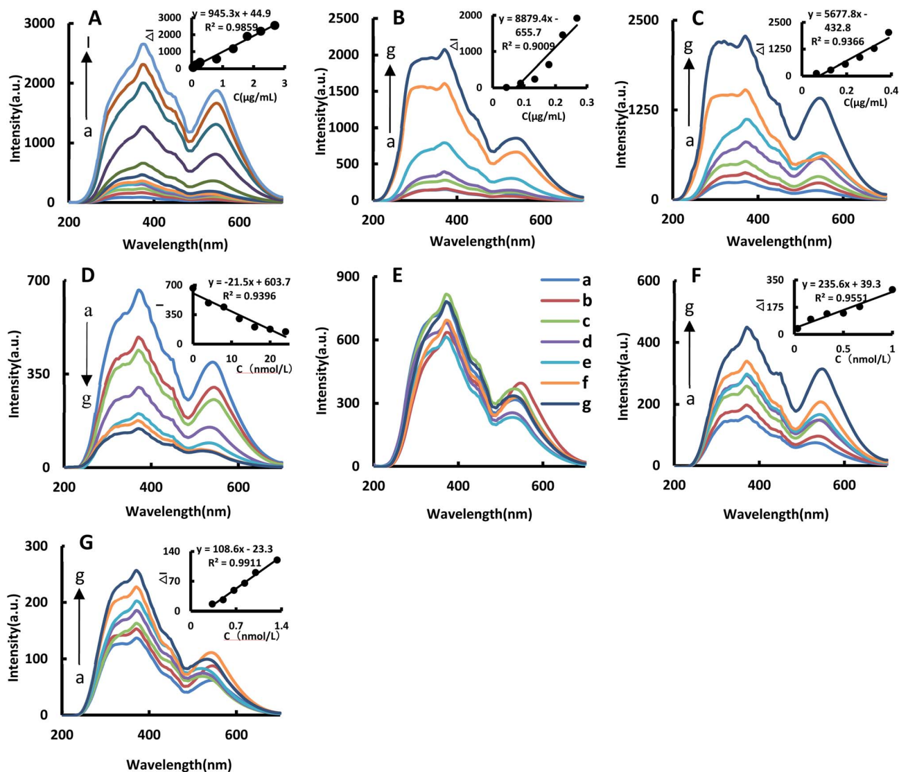
Fig. 4 RRS spectra of the catalytic system. (A): 0.067 \text{ mg mL}^{-1} \text{ HAuCl}_4 + 0.67 \text{ mmol L}^{-1} \text{ HCl} + 3 \text{ mmol L}^{-1} \text{ CHO}_2\text{Na} , (a–l) were 0, 0.044, 0.089, 0.134, 0.179, 0.223, 0.268, 0.804, 1.34, 1.79, 2.23 and 2.68 \mu\text{g mL}^{-1} BtPD, respectively. (B): 0.067 \text{ mg mL}^{-1} \text{ HAuCl}_4 + 0.67 \text{ mmol L}^{-1} \text{ HCl} + 3 \text{ mmol L}^{-1} \text{ CHO}_2\text{Na} , (a–g) represent 0, 0.044, 0.089, 0.134, 0.179, 0.223 and 0.268 \mu\text{g mL}^{-1} AuBtPD, respectively. (C): 0.067 \text{ mg mL}^{-1} \text{ HAuCl}_4 + 0.67 \text{ mmol L}^{-1} \text{ HCl} + 3 \text{ mmol L}^{-1} \text{ CHO}_2\text{Na} , (a–g) represent 0, 0.065, 0.129, 0.194, 0.259, 0.323 and 0.388 \mu\text{g mL}^{-1} AuNPs, respectively. (D): 0.067 \text{ mg mL}^{-1} \text{ HAuCl}_4 + 0.67 \text{ mmol L}^{-1} \text{ HCl} + 3 \text{ mmol L}^{-1} \text{ CHO}_2\text{Na} + 0.145 \mu\text{g mL}^{-1} AuNPs, (a–g) represent 0, 66.67, 133.3, 6.67, 13.3, 0.67 and 1.33 \text{ nmol L}^{-1} Apt, respectively. (E): 0.067 \text{ mg mL}^{-1} \text{ HAuCl}_4 + 0.67 \text{ mmol L}^{-1} \text{ HCl} + 3 \text{ mmol L}^{-1} \text{ CHO}_2\text{Na} + 0.179 \mu\text{g mL}^{-1} AuBtPD, (a–g) represent 0, 4, 8, 12, 16, 20 and 24 \text{ nmol L}^{-1} Apt, respectively. (F): 0.064 \text{ mg mL}^{-1} \text{ HAuCl}_4 + 0.67 \text{ mmol L}^{-1} \text{ HCl} + 3 \text{ mmol L}^{-1} \text{ CHO}_2\text{Na} + 0.179 \mu\text{g mL}^{-1} AuBtPD + 16 \text{ nmol L}^{-1} Apt, (a–g) represent 0, 0.033, 0.167, 0.333, 0.5, 0.667 and 1 \text{ nmol L}^{-1} \text{ Co}^{2+} , respectively. (G): 0.064 \text{ mg mL}^{-1} \text{ HAuCl}_4 + 0.67 \text{ mmol L}^{-1} \text{ HCl} + 3 \text{ mmol L}^{-1} \text{ CHO}_2\text{Na} + 0.179 \mu\text{g mL}^{-1} BtPD + 16 \text{ nmol L}^{-1} Apt, (a–g) represent 0, 0.333, 0.5, 0.667, 0.833, 1 and 1.333 \text{ nmol L}^{-1} \text{ Co}^{2+} , respectively.
