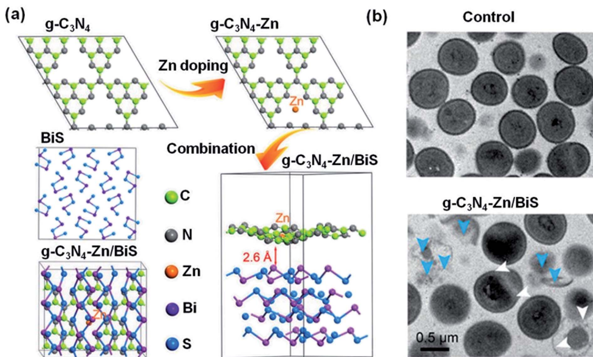
Fig. 8 (a) Structural models of g\text{-C}_3\text{N}_4 , g\text{-C}_3\text{N}_4\text{-Zn} , BiS, and g\text{-C}_3\text{N}_4\text{-Zn/BiS} after geometry optimization. (b) TEM topology of S. aureus after treatment with control or g\text{-C}_3\text{N}_4\text{-Zn/BiS} after 10 min irradiation. The white arrows indicate twisted and broken cell membranes and the blue arrows point to intracellular matrix outflow. Reproduced from ref. 185 with permission from WILEY-VCH, copyright 2019.
