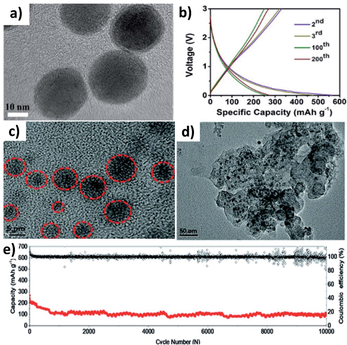
Fig. 7 (a) TEM image and (b) charge–discharge profiles of \text{SnO}_2@3\text{DPDPC} at 100 \text{ mA g}^{-1} . Reproduced with permission. Copyright 2019, Elsevier. (c) HRTEM image of \text{SnO}_2@PC , (d) TEM image of \text{SnO}_2@PC after cycling, and (e) cycling stability of \text{SnO}_2@PC . Reproduced with permission. Copyright 2020, Royal Society of Chemistry.
