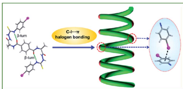
Fig. 9 Schematic illustration of the C-I... \pi halogen bonding driven supramolecular helix. Adapted with permission from ref. 76. Copyright 2017, American Chemical Society.
