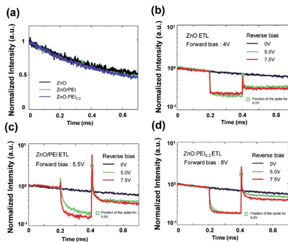
Fig. 7 (a) Delayed EL characteristics of the QDLEDs collected after driving with a forward bias square pulse. The magnitude of the driving voltage was adjusted to achieve a current density of 20 mA cm -2 in all cases ( i.e. 4 V, 5.5 V, and 8 V for the ZnO, ZnO/PEI, and ZnO:PEI 0.3 QDLEDs, respectively). Delayed EL characteristics from the QDLEDs with the ZnO (b), ZnO/PEI (c) and ZnO:PEI 0.3 (d) ETLs showing the effect of applying a 200 \mu s reverse bias pulse with increasing magnitudes on the delayed EL signal. The reverse bias pulse is applied at 0.2 ms.
