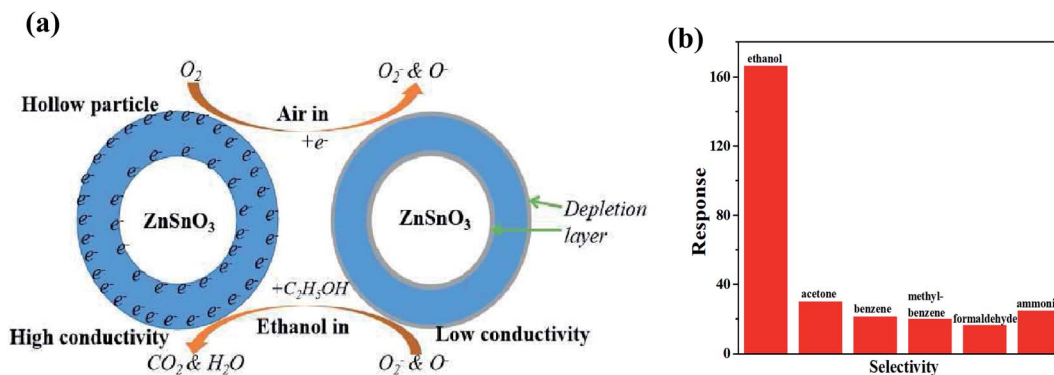
Fig. 17 (a) Ethanol sensing mechanism of ZnSnO 3 hollow particles. (b) Sensing response ( R_3/R_5 ) of CNT@ZnSnO 3 exposed to different types of gases, i.e. ethanol, acetone, benzene, methyl-1-benzene, formaldehyde and ammonia (from left to right) 216 (reprinted from ref. 216, Copyright (2020), with permission from Elsevier).
