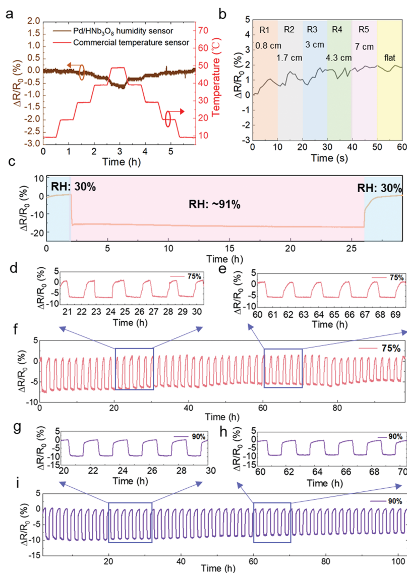
Fig. 4 (a) Temperature dependent test of a 1% Pd/HNb 3 O 8 humidity sensor under temperature variations from 10 ^{\circ}\text{C} to 50 ^{\circ}\text{C} . (b) Real-time bending result of a 1% Pd/HNb 3 O 8 humidity sensor under various bending radii. (c) 24 h stability test of a 1% Pd/HNb 3 O 8 humidity sensor under 90% RH. Long-term stability measurements (50 cycles) under (d–f) 75% RH and (g–i) 90% RH.
