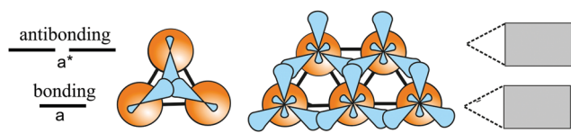
Fig. 4 Energy diagram of three-center bonding with one bonding level, two antibonding levels a^* , and the formation of a 2D network with level broadening to electronic bands and possible formation of a band gap.
