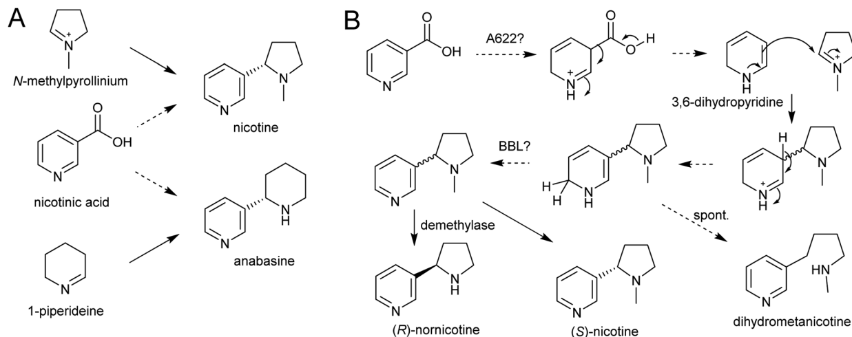
Scheme 21 Nicotine biosynthesis. (A) Origins of nicotine and anabasine. (B) Putative biosynthetic pathway for nicotine.
