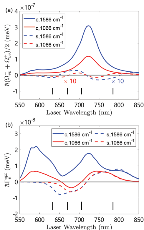
Fig. 5 (a) Vibrational frequency shift (\Omega_{\text{v}}^+ + \Omega_{\text{v}}^-)/2 and (b) effective optomechanical damping rate \Gamma_{\text{v}}^{\text{opt}} = \Gamma_{\text{v}}^- - \Gamma_{\text{v}}^+ as a function of the laser wavelength for the 1586\text{ cm}^{-1} vibrational mode (blue lines) and the 1066\text{ cm}^{-1} vibrational mode (red lines). The solid and dashed lines are the results from the continuum-field model (labeled as “c”) and the single-mode model (labeled as “s”), respectively. The vertical lines indicate wavelengths at 633 nm, 670 nm, 705.9 nm and 785 nm used for later simulations. The laser intensity is 1\text{ }\mu\text{W }\mu\text{m}^{-2} and other parameters are specified in the text.
