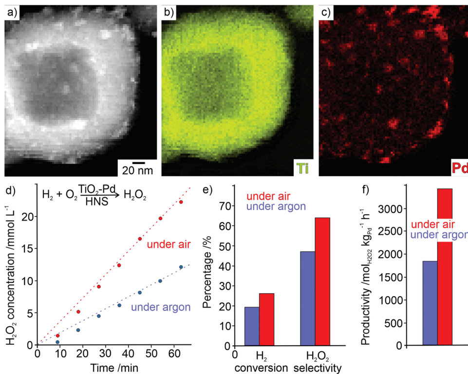
Fig. 5 TiO 2 -Pd HNS (5 wt% Pd) for H 2 O 2 direct synthesis (as-prepared): (a–c) HAADF image (a) with Ti (b) and Pd (c) element mapping; (d–f) H 2 O 2 concentration over time (d), H 2 conversion and H 2 O 2 selectivity (e), H 2 O 2 productivity for catalysts stored under argon (blue) and under air (red).
