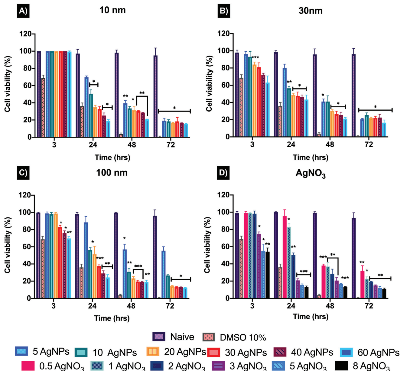
Fig. 3 Viability of embryonic zebrafish cells (ZF4) treated with AgNPs and AgNO 3 for 3, 24, 48 and 72 h. The graphs show the percentage viability of ZF4 cells treated with 5, 10, 20, 30, 40 and 60 \mu\text{g mL}^{-1} of three different AgNPs sizes 10 nm (A), 30 nm (B), and 100 nm (C). Similarly, (D) shows the viability of cells treated with 0.5, 1, 2, 3, 5, and 8 \mu\text{g mL}^{-1} of the ionic control (AgNO 3 ). A positive control of 10% DMSO was also added. Graphs represent the average of three replicates with the standard deviation shown. Data with asterisks (*) indicate a statistically significant difference of the AgNPs treatments (* p < 0.05 , ** p < 0.01 , and *** p < 0.001 ) compared with naïve cells at each time point. All bars under the brackets are included within the asterisk above.
