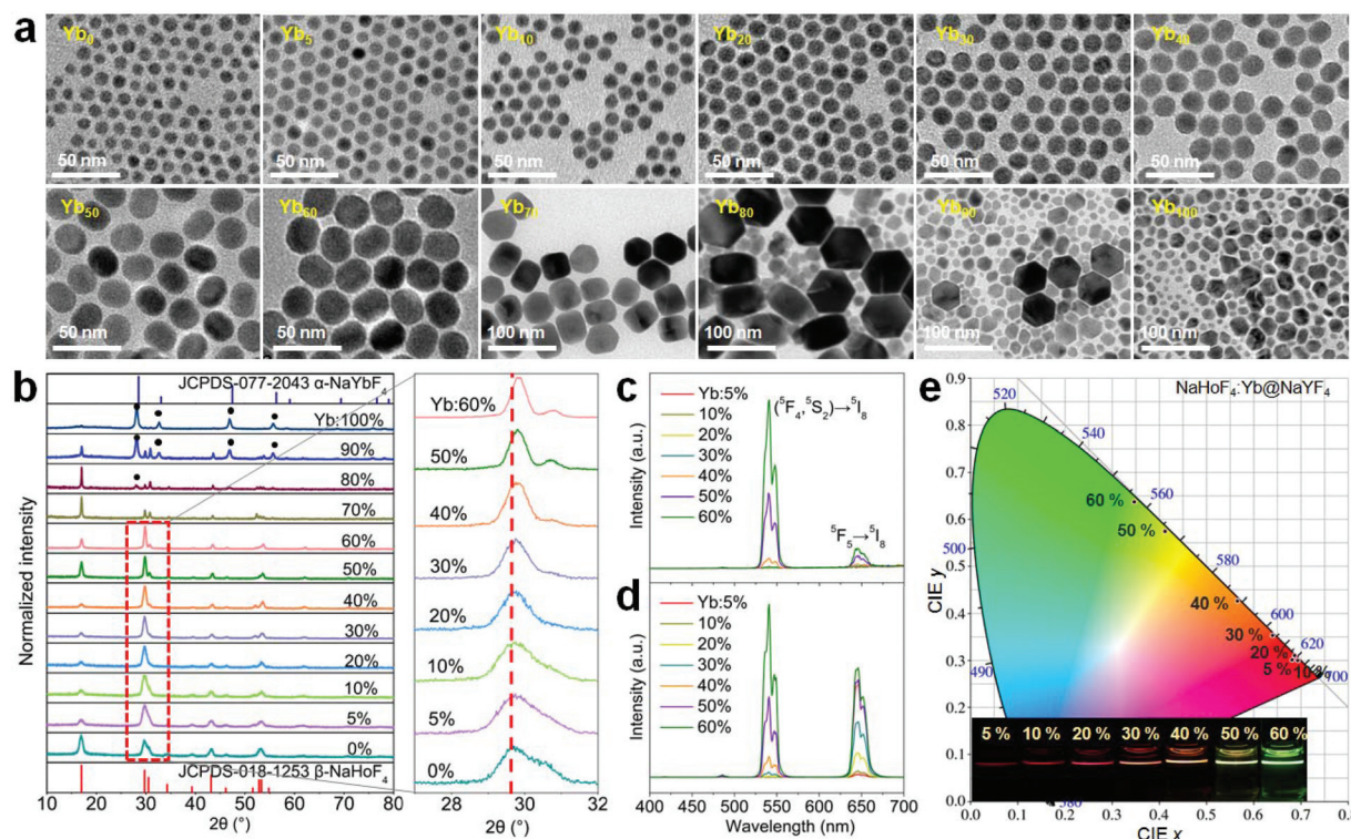
Fig. 2 (a) TEM images of the NaHoF 4 :Yb 3+ (0–100 mol%) core nanoparticles. (b) X-ray diffraction patterns of (a) samples. Inset shows the enlarged (110) diffraction peak for the samples with the Yb 3+ concentration from 0 to 60 mol%. (c and d) Upconversion emission spectra of the as-prepared NaHoF 4 :Yb 3+ (5–60 mol%) core only and NaHoF 4 :Yb 3+ (5–60 mol%)@NaYF 4 core-shell nanoparticles under 980 nm excitation. (e) CIE coordinates of the emissions from (d) samples. Insets show the corresponding emission photographs under 980 nm excitation.
