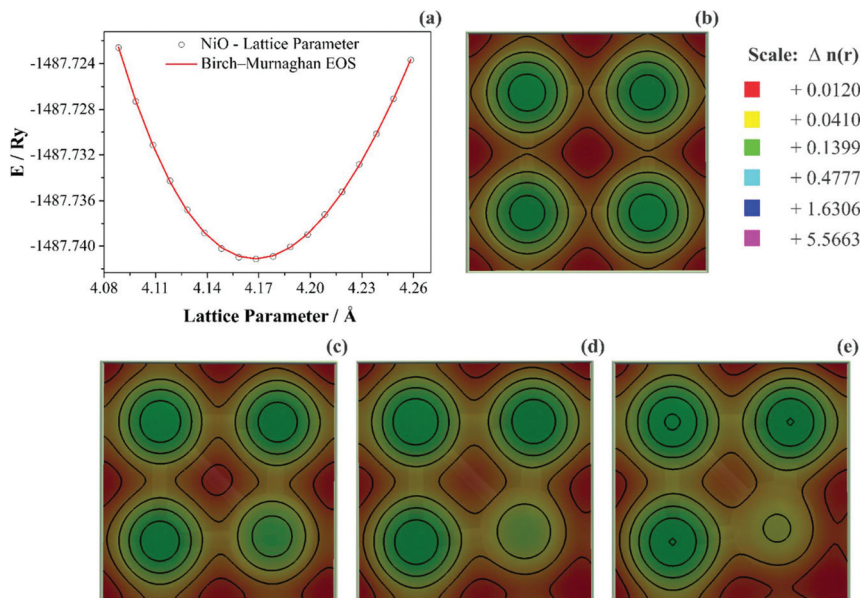
Fig. 7 (a) NiO equation of state (EOS) from DFT-data and Birch–Murnaghan fitting, (b) NiO charge density map using Ni-0.0 Å displacement, (c) Ni-0.02 Å displacement, (d) Ni-0.02 Å displacement, and (e) Ni-0.03 Å displacement.
