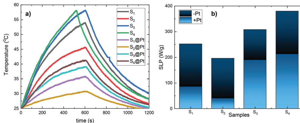
Fig. 6 (a) Heating sequence curves of the PEGylated MNPs and hybrid composites after 600 s of MH treatment and 600 s of sample cooling. The concentration was the same for all samples and equal to 2 mg mL -1 , (b) SLP values of samples before (-Pt) and after (+Pt), the absorption of the complex [Pt(phen)Cl 2 ]. An obvious reduction in SLP is observed for all samples.
