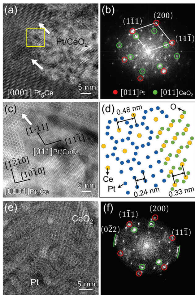
Fig. 5 (a) HRTEM image with [0001]_{\text{Pt}_5\text{Ce}} zone axis and (b) corresponding FFT of the middle separation stage (region 2 in Fig. 3(b)) showing the interface area between \text{Pt}_5\text{Ce} alloy and \text{Pt}/\text{CeO}_2 composites. (c) HAADF-STEM image of the boxed area in (a), and (d) atomic structure model of each phase in the interface area. (e) HRTEM image along the [0001]_{\text{Pt}_5\text{Ce}} zone axis and (f) corresponding FFT of the late separation stage (region 3).
