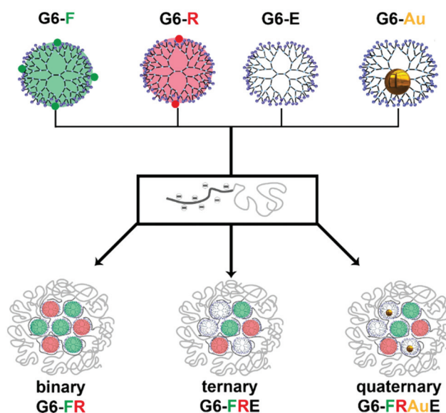
Scheme 1 Schematic overview showing the conversion of regular 6th generation PAMAM (G6-E) into fluorescent fluorescein-functionalized (G6-F), rhodamine B-functionalized dendrimers (G6-R), and dendrimers with encapsulated gold nanoparticles (G6-Au). Charge-stoichiometric addition of negatively-charged pMAA 64 - b -PEO 885 block copolymer to the positively charged G6 dendrimers results in the formation of complex coacervate core dendrimicelles. The dendrimicelle core composition can be stoichiometrically tuned by changing the mixing ratio of the four different dendrimers prior to block copolymer addition, resulting in binary-core, ternary-core and quaternary-core micelles. The positive charges present on the dendrimer periphery at pH 7 and the charges inside the micelle cores are omitted for clarity reasons. It is important to note that the cartoon of the binary/ternary/quaternary-core structures represents the respective dendrimicelle dimensions and its subcomponents approximately on the same relative scale. The cross section of the dendrimicelles shows 7 dendrimers in close proximity, which in a spherical dendrimicelle core containing about 30 dendrimers is in fact the expected ball-park number; also the overall sizes of the dendrimicelle (50 nanometer diameter: 10 nanometer shell and 30 nanometer core) are on relative scale with the dendrimers; useful to comment that the dendrimers perhaps are slightly more spaced and of course in solution are dynamic.
