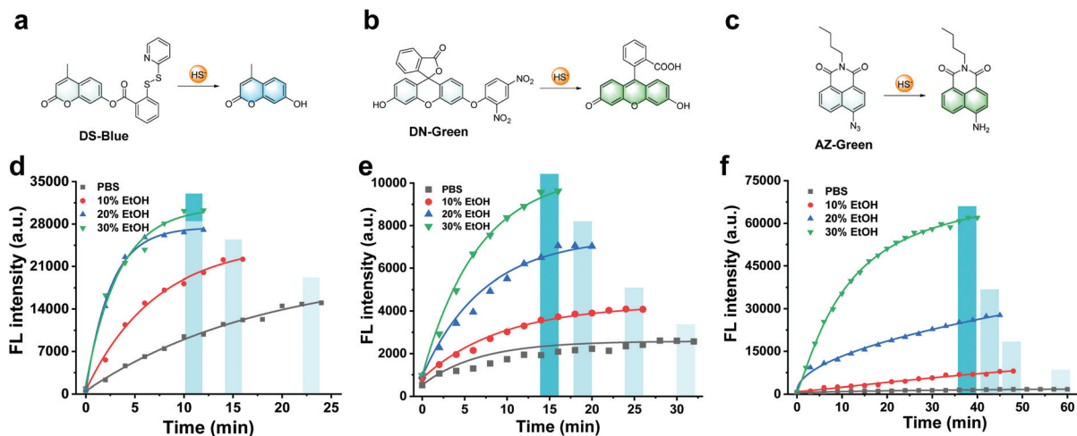
Fig. 1 Co-solvent effect on the reaction time of fluorescent probes to H 2 S. (a–c) Chemical structure and the detection mechanism of DS-Blue, DN-Green, and AZ-Green. (d) Time course of DS-Blue (10 \mu M) with the addition of 20 equivalents H 2 S. (e) Time course of DN-Green (10 \mu M) with the addition of 20 equivalents H 2 S. (f) Time course of AZ-Green (10 \mu M) with the addition of 20 equivalents H 2 S. Solutions are PBS, 10% ethanol, 20% ethanol, and 30% ethanol in PBS (10 mM, pH 7.4, v/v), respectively.
