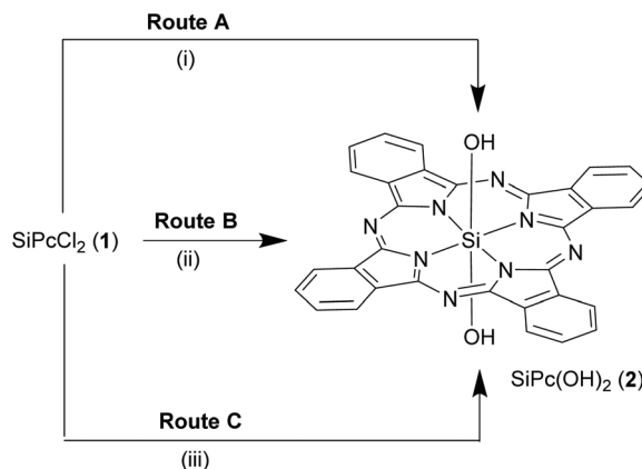
Scheme 3 Synthetic routes for hydrolysis of the axial chloro bonds to form bis-hydroxyl SiPc derivative, 2 . Reagents and conditions: (i) 1:1 (v/v) pyridine and conc. aq. NH 3 , 10 h, reflux; (ii) large excess of conc. H 2 SO 4 , r.t.; (iii) NaOCH 3 , 95% ethanol, reflux, 1 h.
