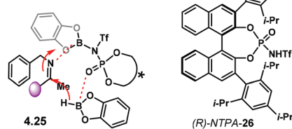
Scheme 47 (a) Asymmetric reduction of ketimines using catecholborane. (b) Proposed bifunctional activation mode. Herein, the NTPA-borane complex serves as the catalytic species.
