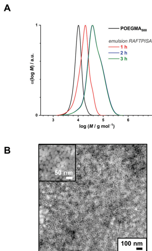
Fig. 2 (A) Size-exclusion chromatograms of polymers obtained by PBBMA emulsion RAFTPISA in water/ethanol 3 : 1 vol/vol at 70 °C with POEGMA_{500} at DP_{th} = 100 , and 20 wt% solids content (entry 4 from Table S2 † ). (B) Transmission electron micrograph of nanoparticles obtained in the conditions mentioned above, after 2 h.
