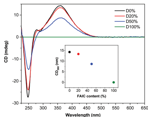
Fig. 3 CD ( \text{THF} , 0.5 \text{ mg mL}^{-1} ) spectra of P(\text{PAIC})_{20}\text{-}b\text{-}(P(\text{MAIC})_y\text{-}co\text{-}P(\text{FAIC})_z)_{30} with 0, 20, 50 and 100 mol% of FAIC .
