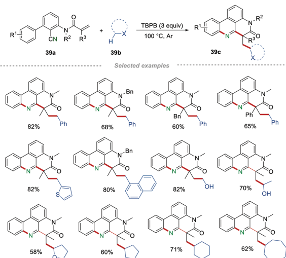
Scheme 39 The construction of alkyl-substituted phenanthridines.
