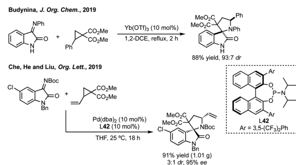
Scheme 42 Selected examples of 3,2'-spirooxindole synthesis by cyclopropane ring expansion.
