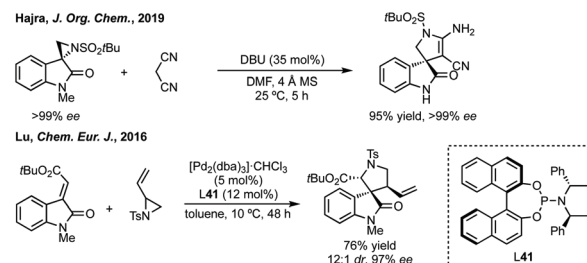
Scheme 41 3,3'-Spirooxindoles synthesised by aziridine ring expansion.
