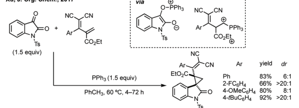
Scheme 4 P(NMe 2 ) 3 -mediated reductive cyclopropanation via Kukhtin-Ramirez (K-R) adduct and K-R adduct reaction with diene activated by PPh 3 .
