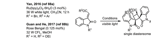
Scheme 18 [2 + 2]-Photocycloaddition of 3-ylideneoxindoles.
