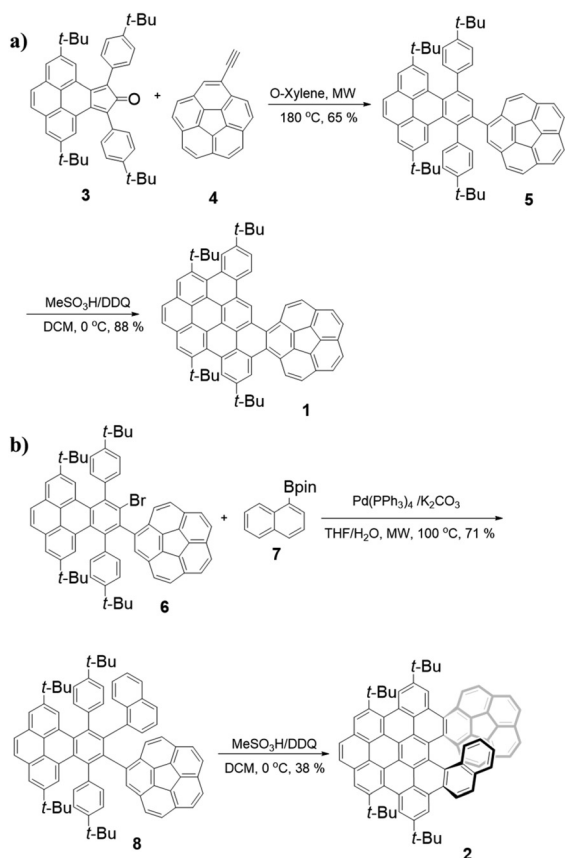
Scheme 1 Synthetic routes of 1 (a) and 2 (b).
